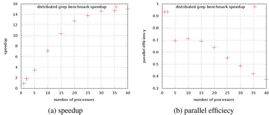
Fig. 2: distributed grep benchmark speedup and parallel efficiency plots
